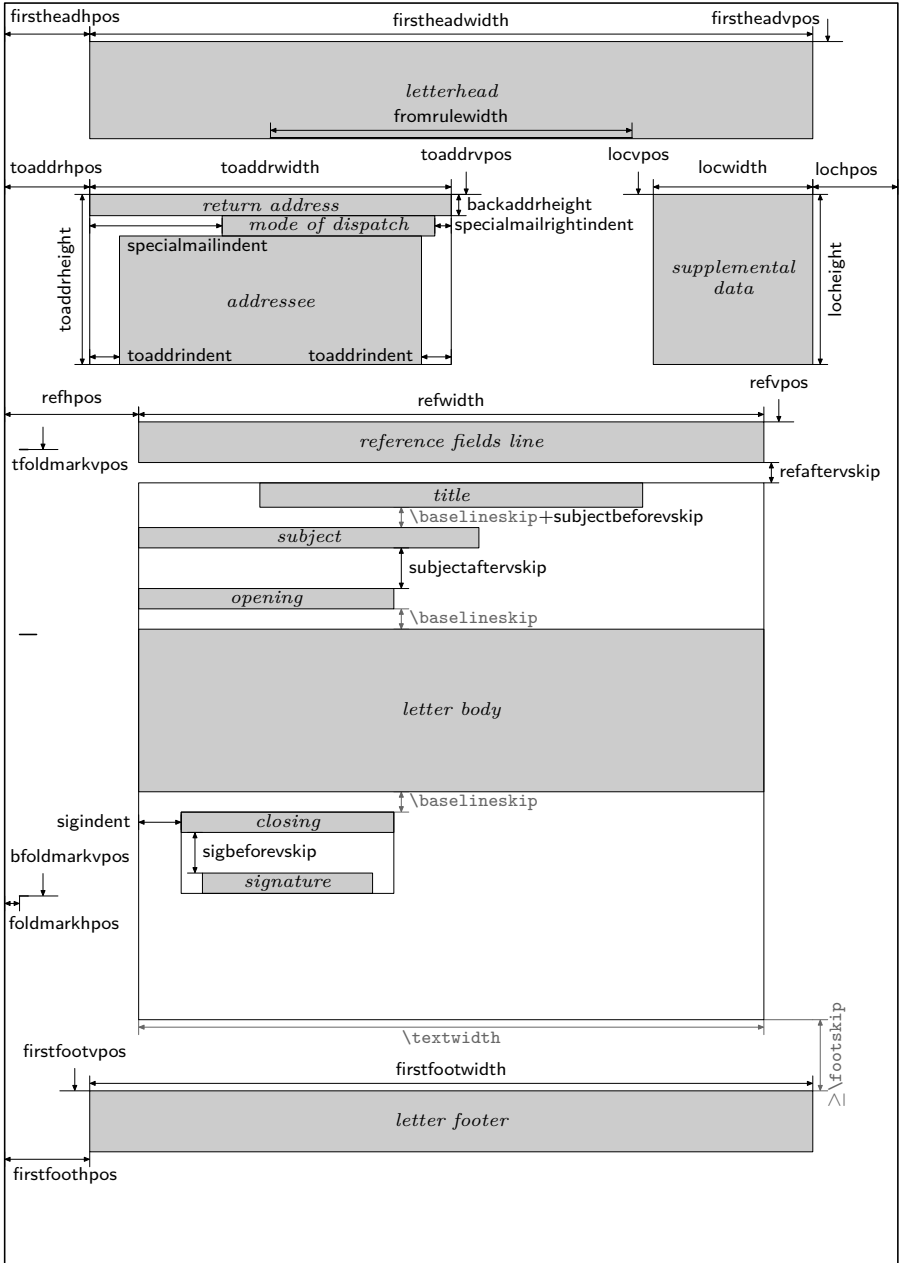
Figure 6.1.: Schematic of the pseudo-lengths for a letter
